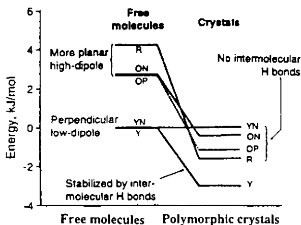
Fig. 4. Comparison of conformational energies and crystal energies of the various polymorphs of 5-methyl-2-[2-(nitrophenylamino)-3-thiophenecarbonitrile (II). Form R (red prisms, m.p. 106.2°C), form Y (yellow prisms, m.p. 109.8°C), form OP (orange plates, m.p. 112.7°C), form ON (orange needles, m.p. 114.8°C), form YN (yellow needles, m.p. not measurable) ([42], reproduced with the permission of the American Chemical Society).
