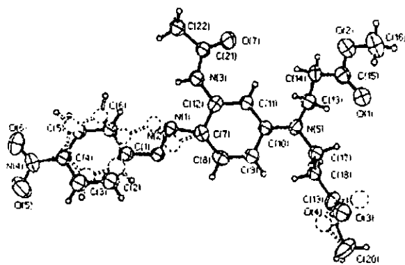
Fig. 5. ORTEP plots of the two molecular conformations (1 and 2) for the X-ray structure determination of 2'-acetamido-4'-[ N,N -bis(2-methoxycarbonyl)ethoxy]amino]-4-nitroazobenzene (Scheme 1 Structure) at 293 K. Thermal ellipsoids are shown at 30% for clarity, with conformer 2 being represented by the solid lines and Conformer 1 by the dotted lines ([48], reproduced with the permission of the American Chemical Society).
