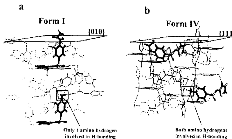
Fig. 7. Possible binding interaction of ethamidiosulfamide in the fastest growing faces of (a) form I and (b) form IV of sulfathiazole ([59], reproduced with the permission of Elsevier Science).
