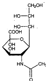
N -Acetylneuraminic acid
