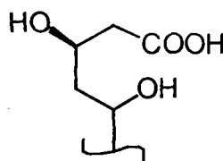
Dihydroxy Open-Acid
