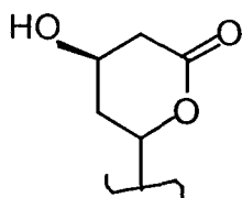
Lactone
