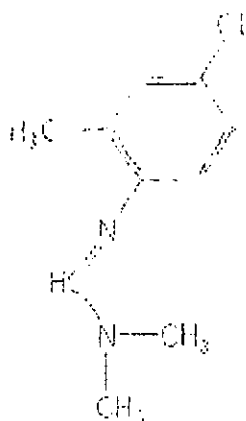
Clordimeform
