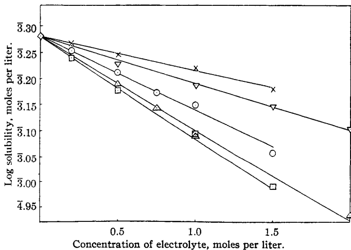
Fig. 2.—Solubilities of molecular m -chlorobenzoic acid in salt solutions: ×, NaClO 4 ; ○, KCl; Δ, NaCl; ∇, KBr; □, LiCl.
