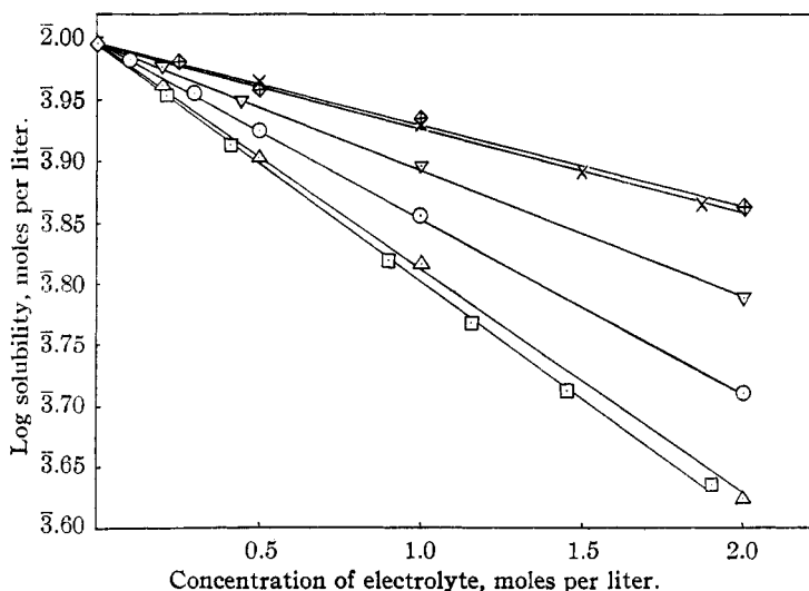
Fig. 1.—Solubilities of molecular o -chlorobenzoic acid in salt solutions: ×, NaClO 4 ; ∇, KBr; ○, KCl; Δ, NaCl; □, LiCl; ⊕, CsCl.
