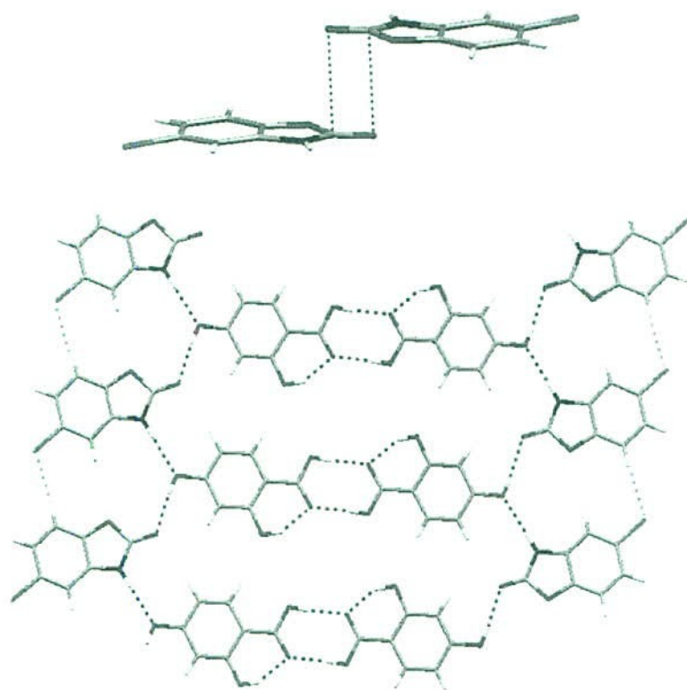
Fig. 21 Anti-parallel centrosymmetric carbonyl–carbonyl interaction between two molecules ( top ) and the packing motif ( bottom ) of chlorzoxazone in co-crystal form I. Repulsive C–H...Cl–C interactions are in light grey .
