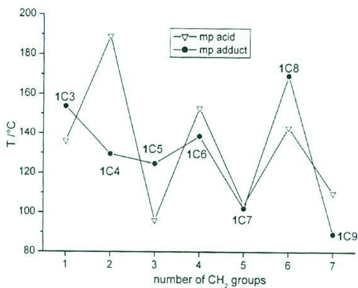
Fig. 17 Melting point alternation in neutral acids and in compounds 1C3–1C9
