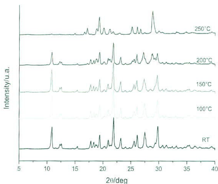
Fig. 11 XRPD recorded at different temperatures from room temperature to 250°C on crystalline \text{NH}_4(\text{C}_4\text{H}_3\text{N}_2\text{O}_3) showing the presence of new reflections at 200°C
