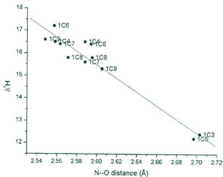
Fig. 16 Compact view of ^1\text{H} chemical shifts as a function of N...O distance
