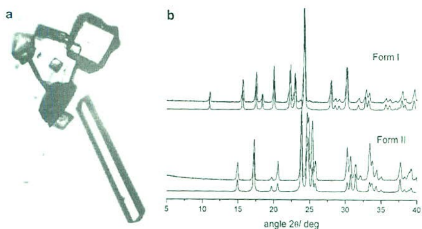
Fig. 4 Concomitant polymorphs obtained from an ethanol/water solution; rods form I, blocks form II a Comparison between the experimental and calculated powder diffractograms of form I and form II b
