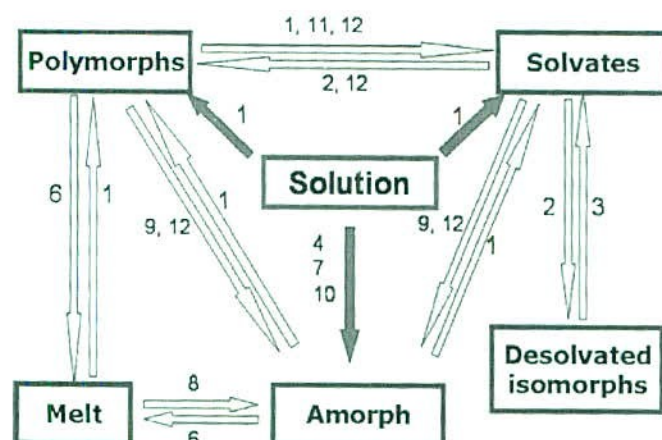
Fig. 3 Some general relationships between polymorphs, solvates and amorphous phases and the type of research laboratory or industrial or process for preparation and interconversion: 1 crystallization; 2 desolvation; 3 exposure to solvent/vapour uptake; 4 freeze drying; 5 heating; 6 melting; 7 precipitation; 8 quench cooling; 9 milling; 10 spray drying; 11 kneading; 12 wet granulation. Analogous relationships apply to polymorphic modifications of solvate forms. Note that the figure represents general trends rather than every possible transformation; the presence or absence of an arrow or number does not represent the exclusive existence or absence of a transformation
