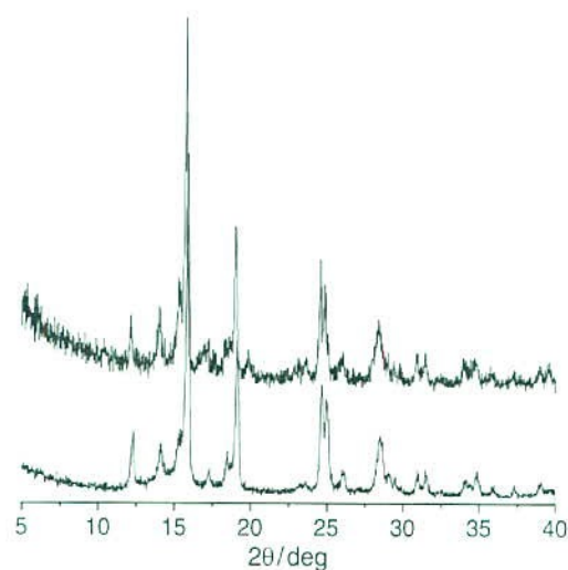
Fig. 12 Comparison between the experimental powder diffractograms of compound 1, obtained from the solid–gas reaction with ammonia of form I ( top ) and form II ( bottom ), respectively
