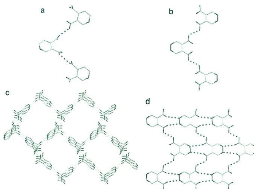
Fig. 5 Chains present in form I a and form II b ; the adamantoid network formed by N–H...O– hydrogen bonds among the chains and the overall crystal structure formed by the three interpenetrating networks in form I c ; interactions N–H...O– and C–H...O– among the chains and the 2D-network present in form II d
