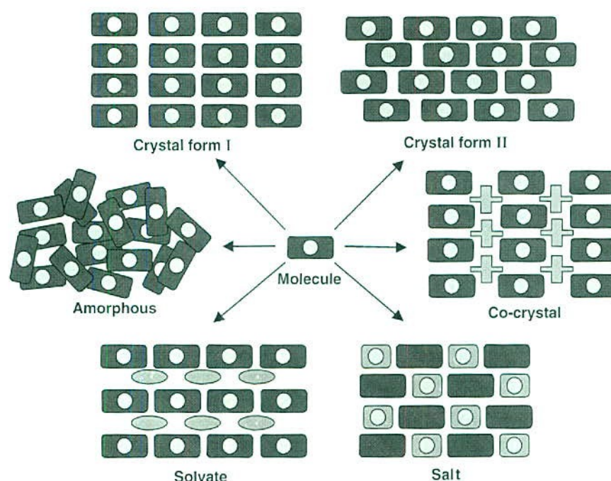
Fig. 1 Schematic representation of the structural relationship between “true” polymorphs, solvates, co-crystals, salts and the amorphous phase
