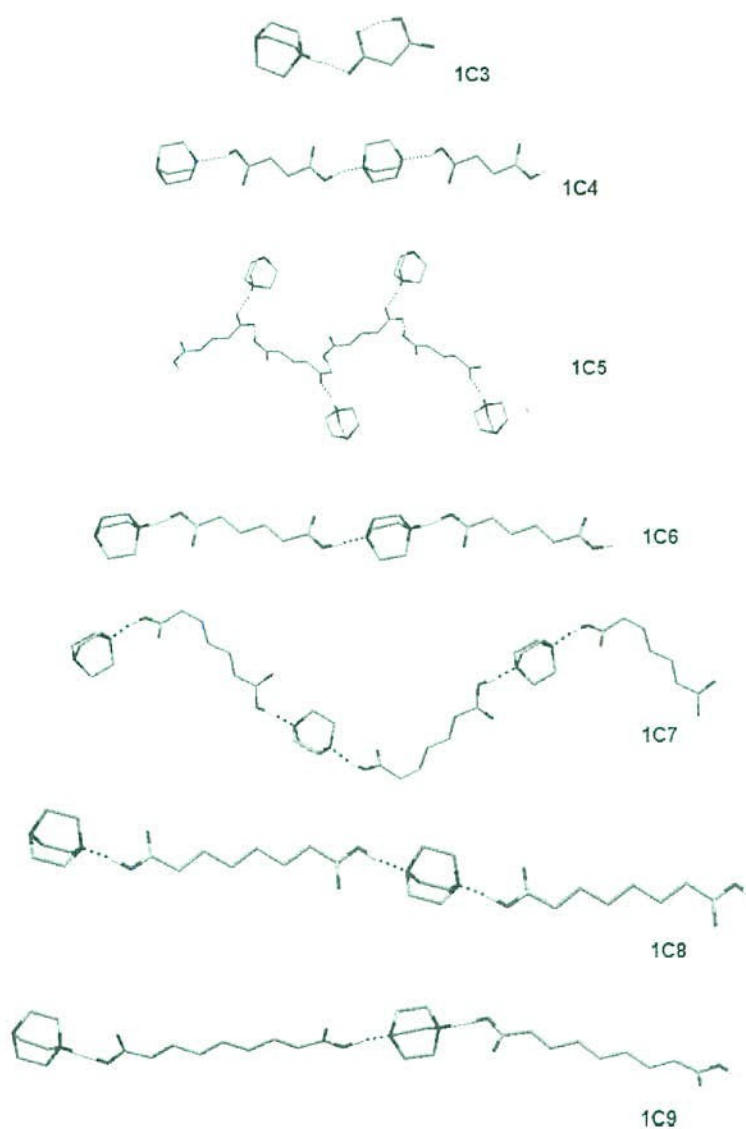
Fig. 15 Schematic representation of the packing motives in [N(CH_2CH_2)_3N^+H][OOC(CH_2)_nCOO^-] ( n = 1-7 , i.e. 1C3 , 1C4 , 1C5 , 1C6 , 1C7 , 1C8 , and 1C9 )
