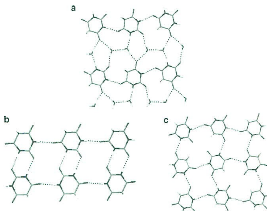
Fig. 9 Hydrogen bond networks present in the dihydrate form a , form I b and form II c of barbituric acid
