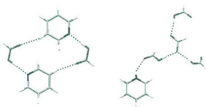
Fig. 14 The 1:1 co-crystal of pyridine and formic acid where the proton transfer does not occur ( left ) and the 1:4 co-crystal of pyridine and formic acid where the formate anion is present ( right )
