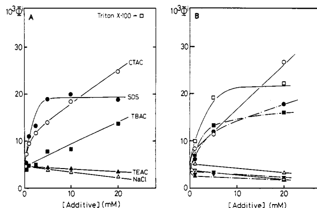
Figure 3. (A) Dependence of the initial quantum yield \Phi^i on the concentration of additives in MPTH-MV 2+ systems. (B) Dependence of the initial quantum yield \Phi^i on the concentration of additives in ionic PTH-MV 2+ systems. QPTH3-MV 2+ : (○) CTAC, (□) SDS, (Δ) TEAC, (▽) NaCl. SPTH3-MV 2+ : (●) CTAC, (■) SDS, (▲) TEAC, (▼) NaCl.
