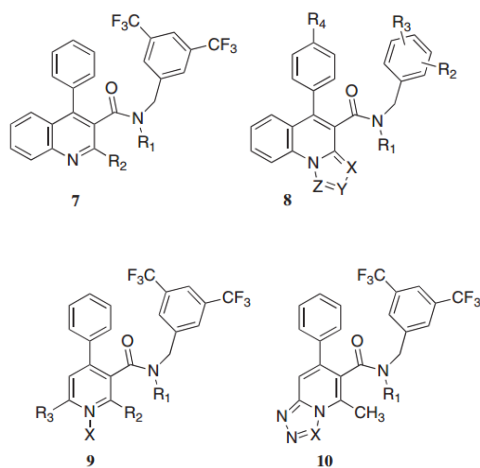
Figure 2. Structures of NK 1 receptor ligands 7–10 from our laboratory.
