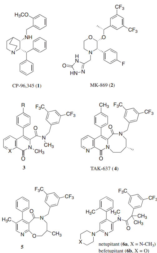
Figure 1. Structures of NK 1 receptor antagonists 1–6 from Pfizer, Merck, Takeda, and Hoffmann-La Roche.
