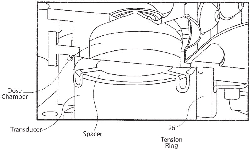
Figure 4: Tension Mechanism showing transducer, dose chamber, spacer and melinex tension ring
