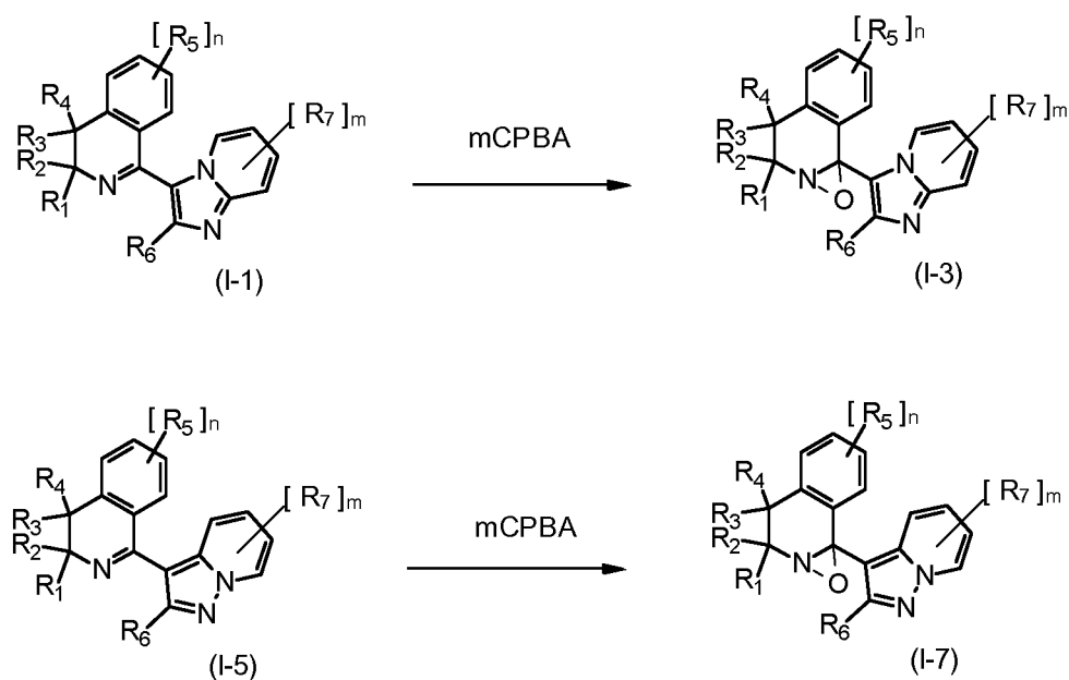
Scheme 28
