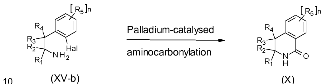
Scheme 11
