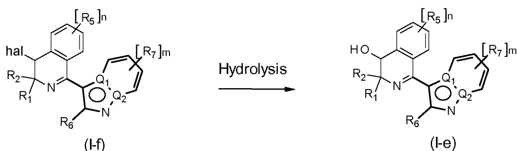
Scheme 21
