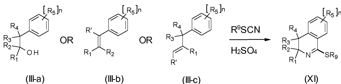
Scheme 6
