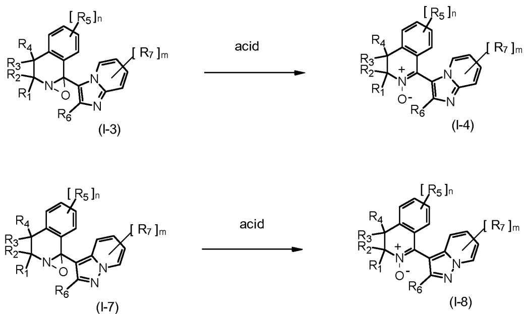
Scheme 30
