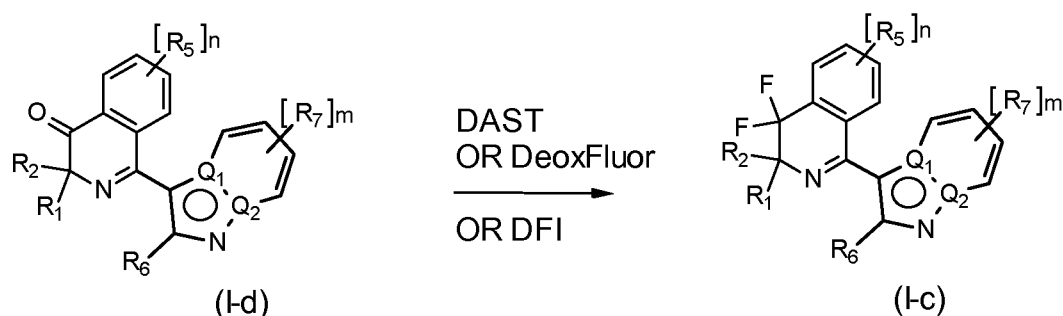
Scheme 19
