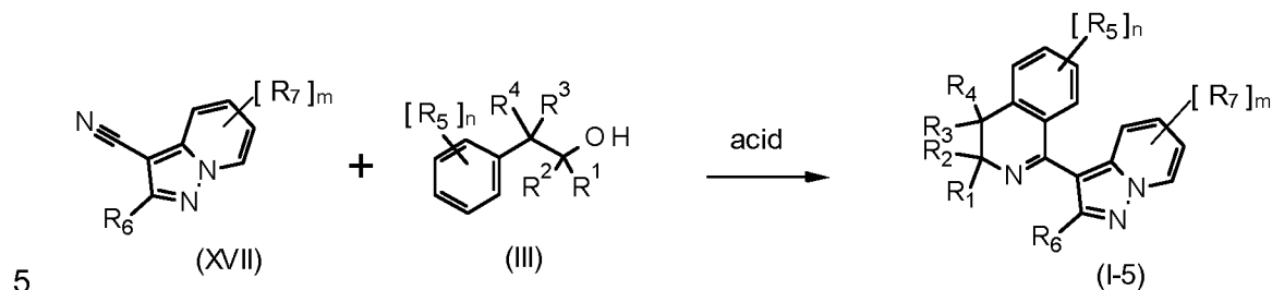
Scheme 13
