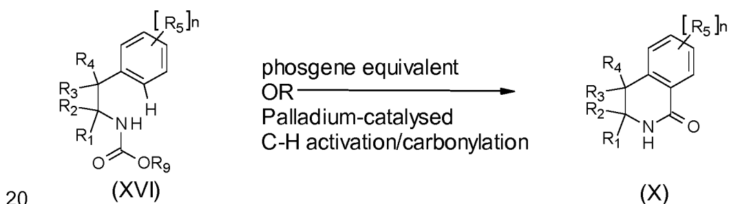
Scheme 12
