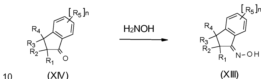
Scheme 9
