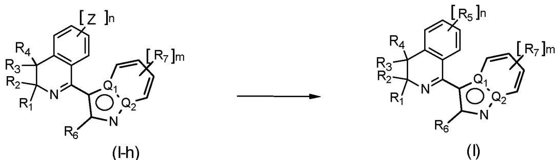
Scheme 25
