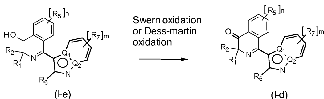
10 Scheme 20
