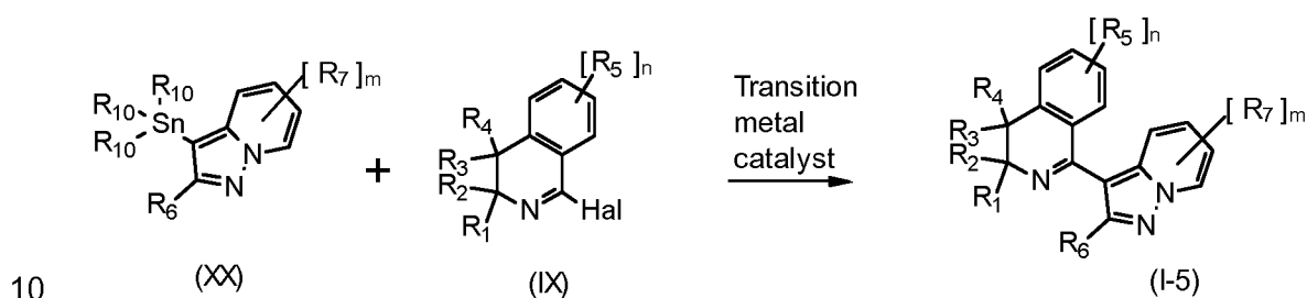
Scheme 16
