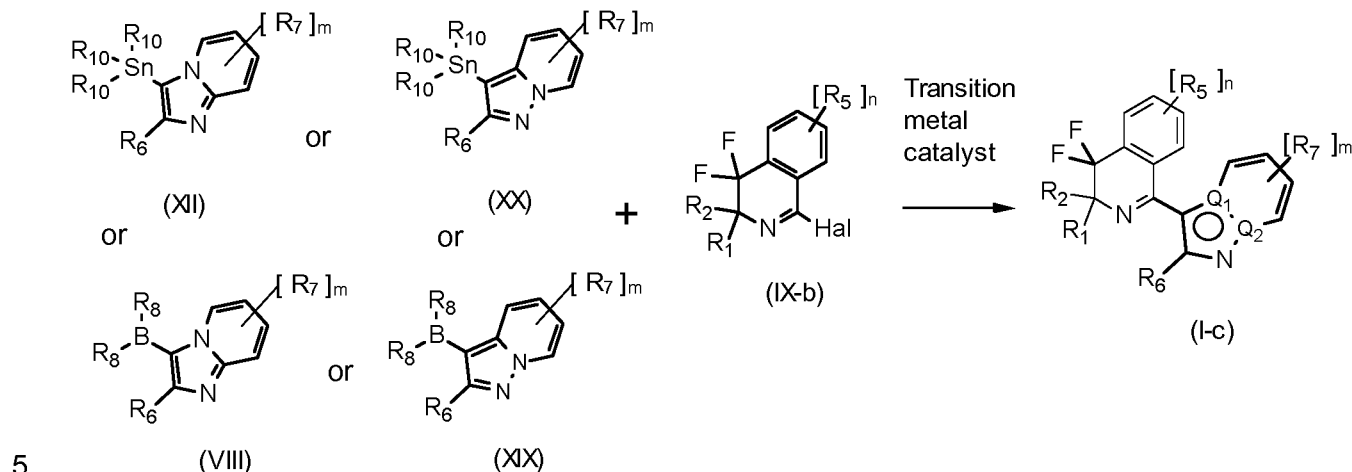
Scheme 24
