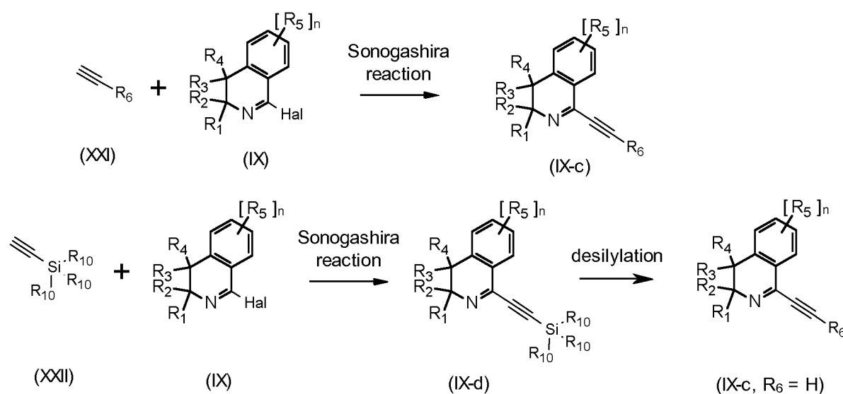
10 Scheme 18
