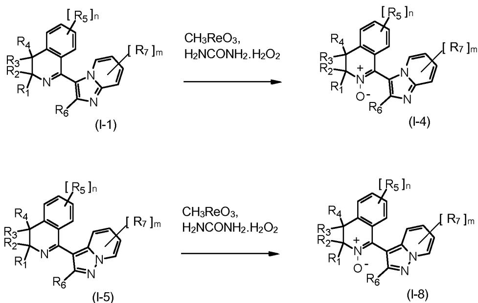
Scheme 29
