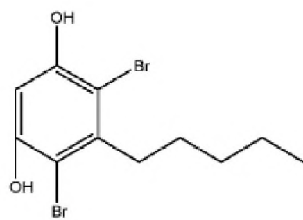
4,6-dibromo-olivetol
