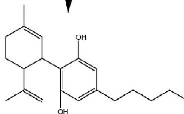
cannabidiol
