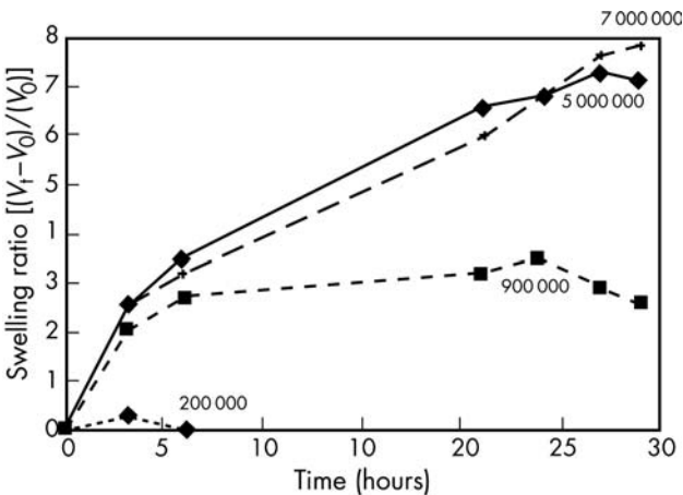
Figure 1: Swelling capacity of polyethylene oxide (Polyox WSR). Measured for four molecular weight grades; 28 mm tablets in 300 mL of water.
