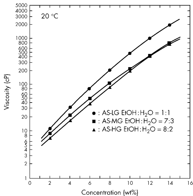
Figure 1: Viscosity of different grades of Aqoat (Shin-Etsu). (4)
