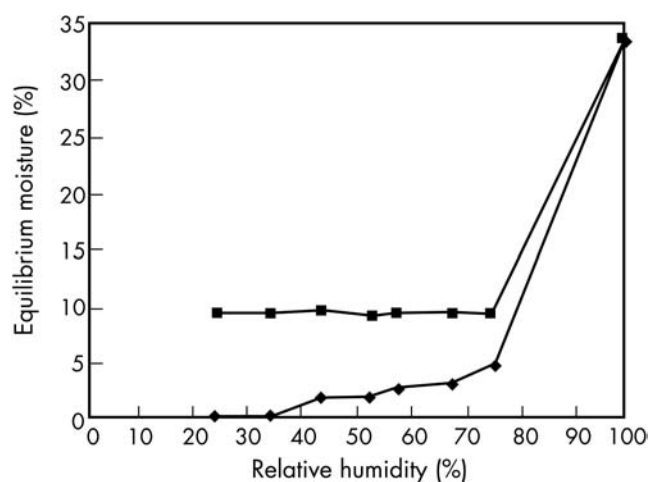
Figure 1: Sorption-desorption isotherm for anhydrous dextrose granules.
