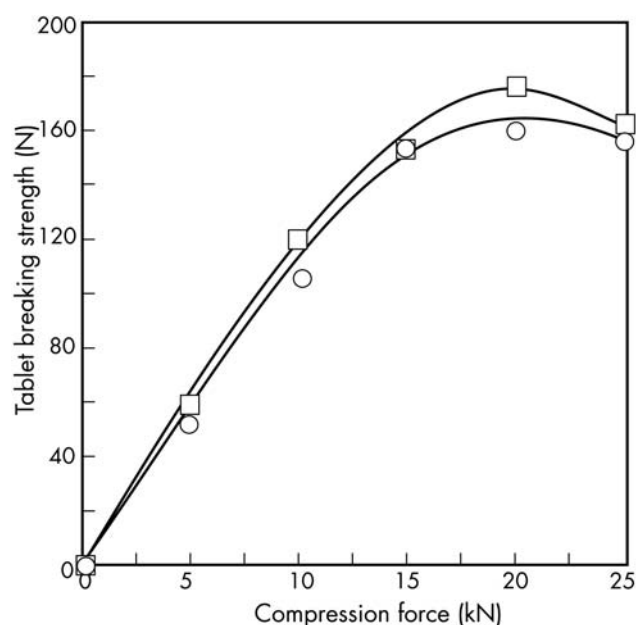
Figure 1: Compression characteristics of Xylitolab 100 and Xylitolab 200 (Danisco Sweeteners Ltd.).
