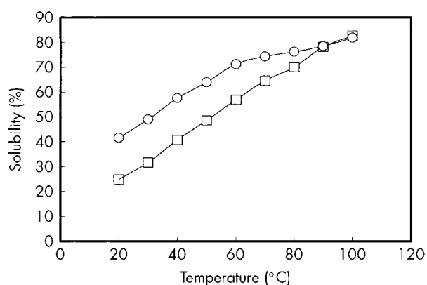
Figure 3: Solubility of isomalt types in water. (2)
