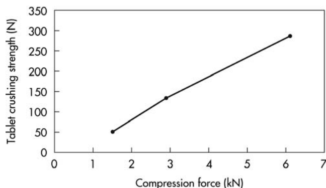
Figure 1: Tablet crushing strength of isomalt (GalenIQ 720, Palatinit GmbH).
