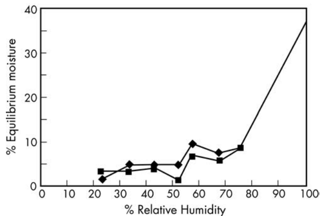
Figure 1: Absorption-desorption isotherm for hypromellose.
