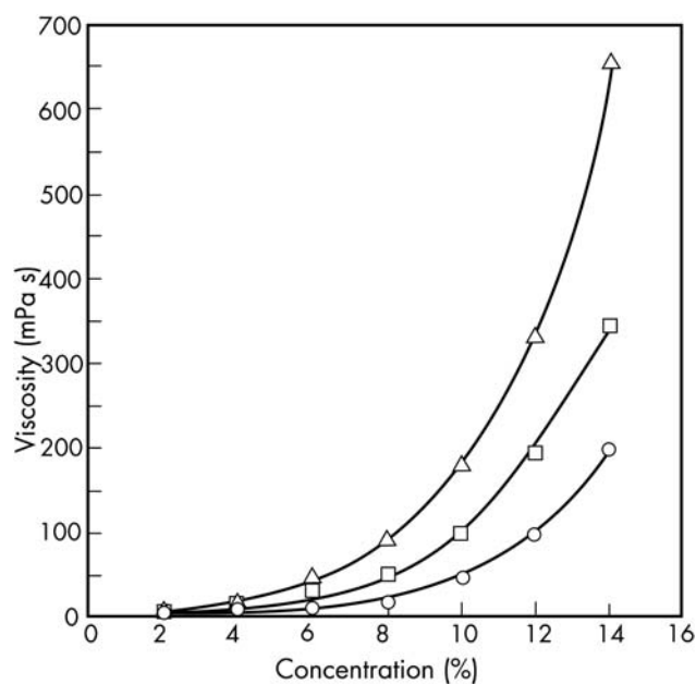
Figure 3: Dynamic viscosity of hypromellose phthalate (HP-50) (Shin-Etsu Chemical Co. Ltd.) in various solvent mixtures at 20°C. (11) ○: Acetone: ethanol (1:1) □: Dichloromethane: ethanol (1:1) △: Ethanol: water (1:1)
