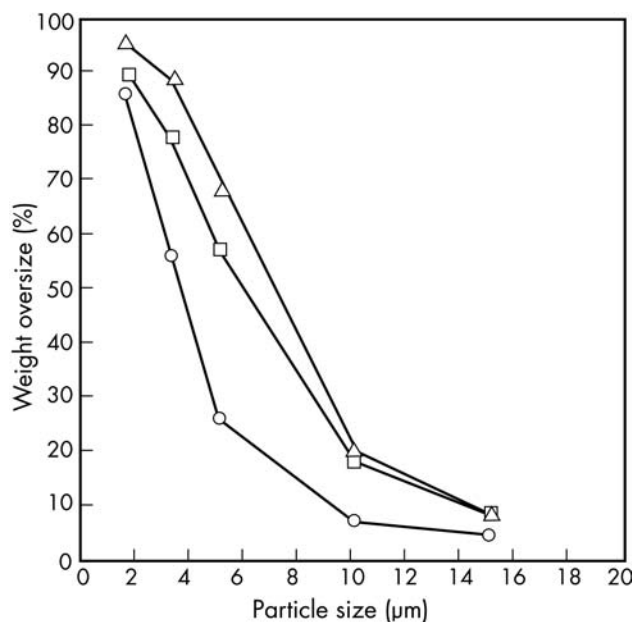
Figure 2: Particle-size distribution of calcium carbonate (Sturcal, Rhodia).
