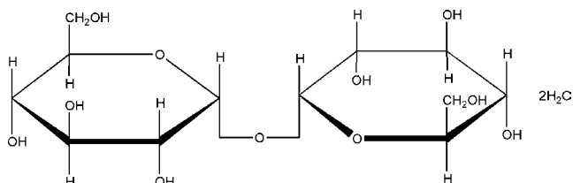
\alpha,\alpha -Trehalose dihydrate
