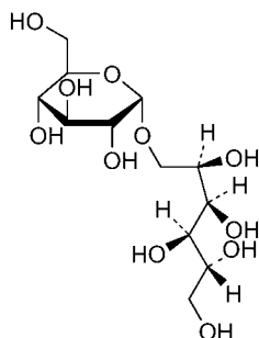
C_{12}H_{24}O_{11} (1,6-GPS)
