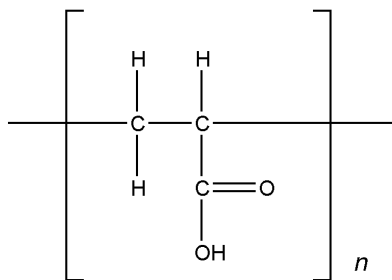
Acrylic acid monomer unit in carbomer resins.
