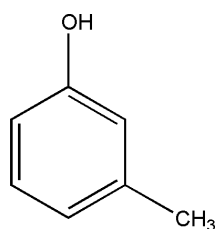
m -Cresol
