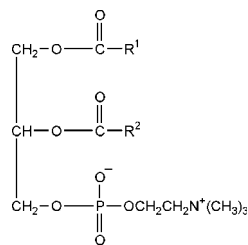
\alpha -Phosphatidylcholine
