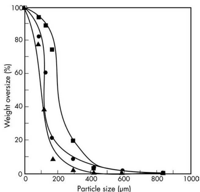
Figure 3: Particle size distribution of granulated xylitol (Xylitab, Danisco Sweeteners Ltd.). ●: Xylitab 100 granulated with 3.5% polydextrose ■: Xylitab 200 granulated with 2.0% carboxymethyl-cellulose ▲: Xylitab 300 wet granulated.
