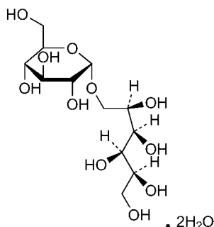
C_{12}H_{24}O_{11} \cdot 2H_2O (1,1-GPM)
