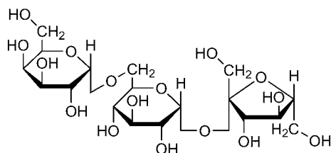
D-Raffinose anhydrous
