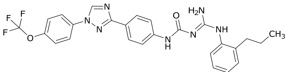
(1E)-1-[Amino-(2,5-dimetilanilino)metileno]-3-[4-[1-[4-(trifluorometoxi)fenil]-1H-1,2,4-triazol-3-il]fenil]urea (F7)
