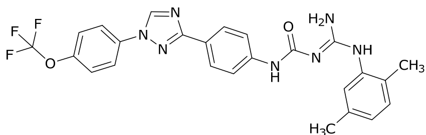
(1E)-1-[Amino-(2,4-dimetilanilino)metileno]-3-[4-[1-[4-(trifluorometoxi)fenil]-1H-1,2,4-triazol-3-il]fenil]urea (F8)
