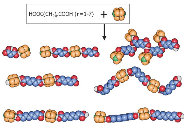
Fig. 6 The reaction of solid dicarboxylic acids \text{HOOC}(\text{CH}_2)_n\text{COOH} ( n = 1\text{--}7 ) with the solid base 1,4-diazabicyclo[2.2.2]octane, [\text{N}(\text{CH}_2\text{CH}_2)_3\text{N}] , generates the corresponding salts or co-crystals of formula [\text{N}(\text{CH}_2\text{CH}_2)_3\text{N}]\text{--H--}[\text{OOC}(\text{CH}_2)_n\text{COOH}] ( n = 1\text{--}7 ). The \text{O--H}\cdots\text{O} hydrogen bonds present in the solid acid are replaced by neutral \text{O--H}\cdots\text{N} and charged (^-)\text{O}\cdots\text{H--N}^{(+)} interactions, with formation of dimeric units ( n = 1 ) or infinite chains ( n = 2\text{--}7 ) ( \text{H}_{\text{CH}} atoms not shown for clarity).
