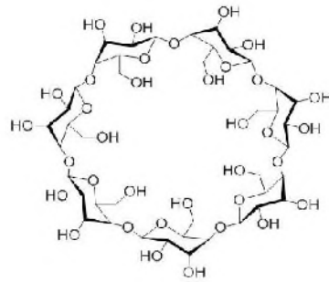
\beta -Cyclodextrin
