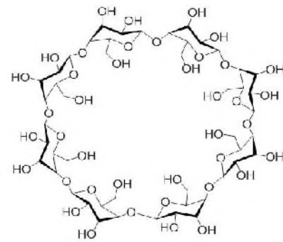
\gamma -Cyclodextrin
