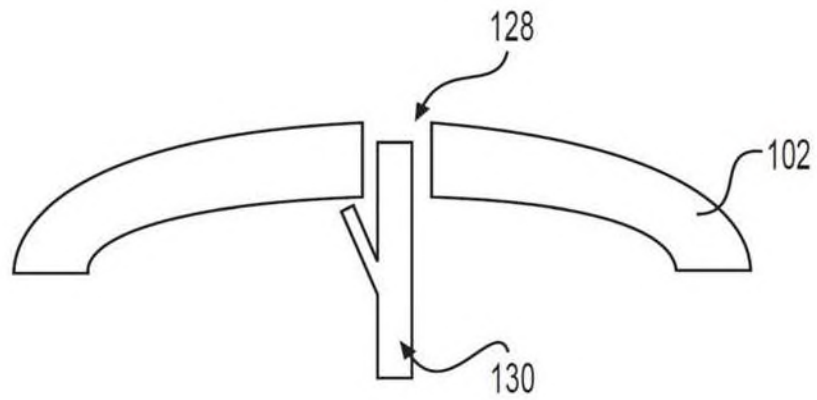
FIGURE 9C
