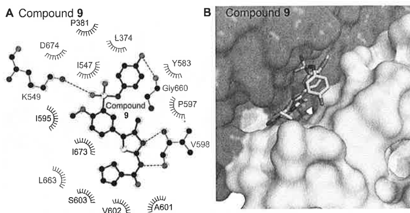
Figure 3. Structural basis of inhibition of PI4KIII \beta by compound 9. (A) Residues mediating the interaction of PI4KIII \beta with compound 9 are shown, with putative hydrogen bonds indicated by dotted lines. Figure generated using LIGPLOT. 43 (B) Fit of compound 9 in the PI4KIII \beta active site pocket. The kinase domain is colored with the N-lobe shown in red and the C-lobe shown in yellow.
