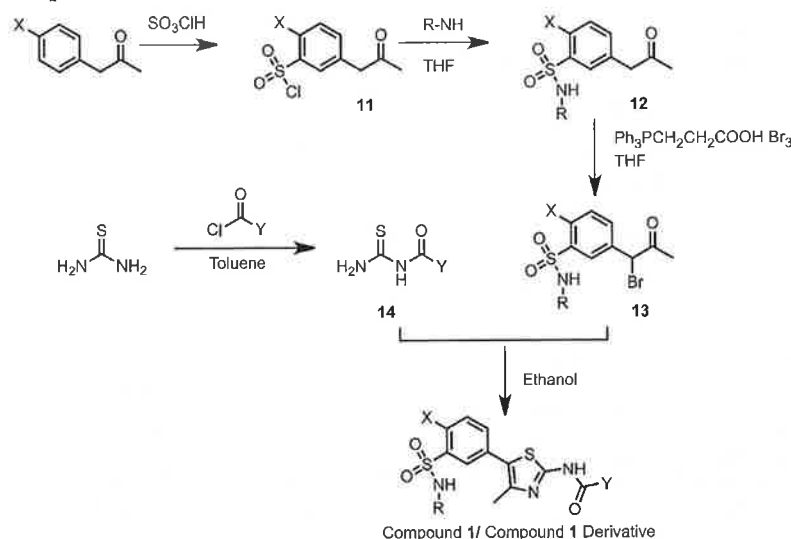
Scheme 1. Synthesis of Compound 1 and Derivatives
