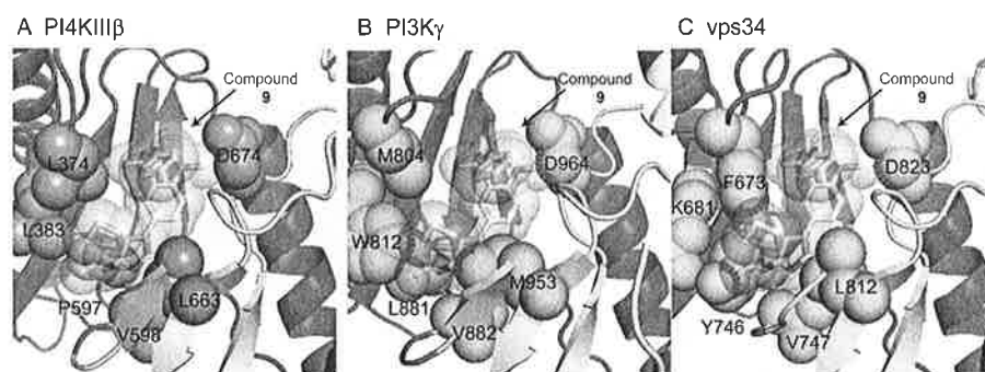
Figure 4. Structural basis for selectivity of compound 9. (A) Structure of compound 9 bound to PI4KIII \beta , with selected residues colored in orange and shown as spheres. (B) Model of compound 9 in the active site of PI3K \gamma . The model was generated by aligning the active site of the structure of compound 9 bound to PI4KIII \beta to the structure of PI3K \gamma bound to compound 1 (PDB ID: 2CHZ). The equivalent residues shown in panel A are colored in green and shown as spheres, with steric clashes highlighted in red. (C) Model of compound 9 in the active site of vps34. The model was generated by aligning the active site of the structure of compound 9 bound to PI4KIII \beta to the structure of vps34 bound to compound 1 (PDB ID: 2X6J). The equivalent residues shown in panel A are colored in cyan and shown as spheres, with steric clashes highlighted in red.
