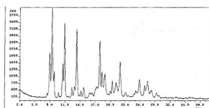
FIG. 1 Form A of 2-methyl-2-[4-(3-methyl-2-oxo-8-quinolin-3-yl-2,3-dihydro-imidazo[4,5-c]quinolin-1-yl)-phenyl]-propanitrile
