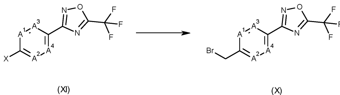
Scheme 9
