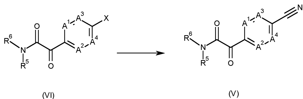
Scheme 4
