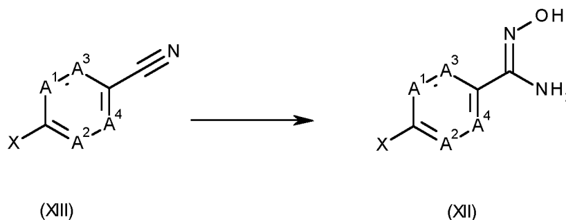
Scheme 12
