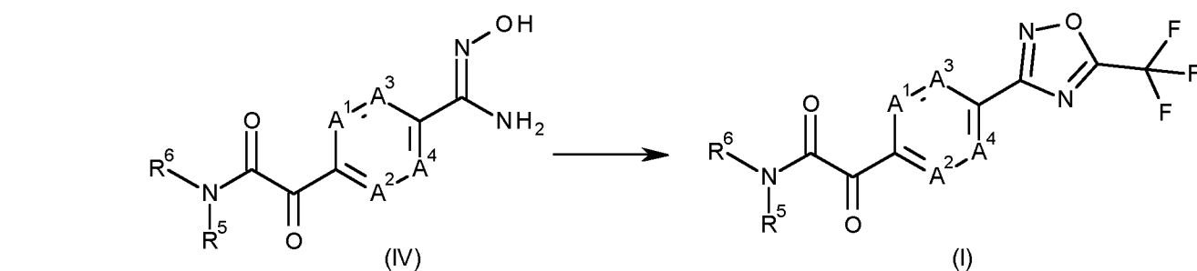
Scheme 2
