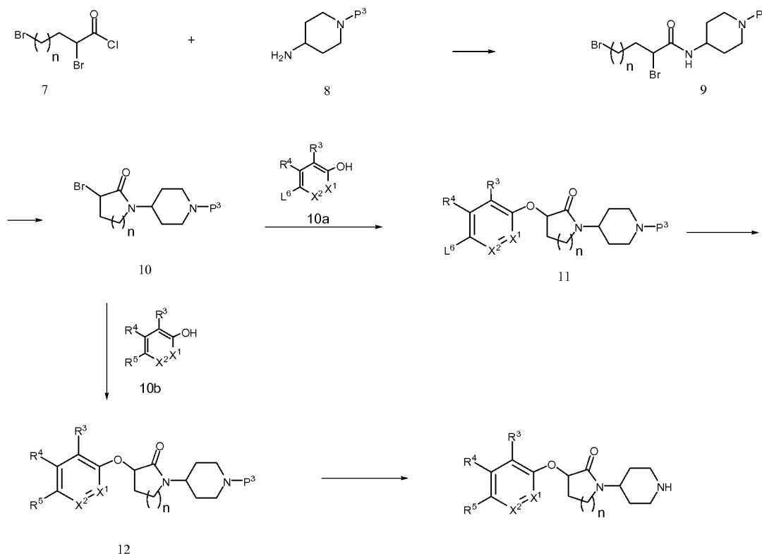
Scheme 2
