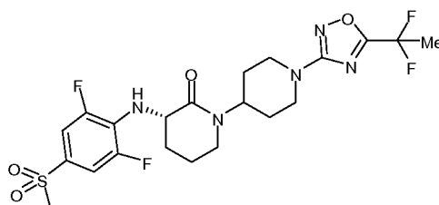
(S)-3-(2,6-difluoro-4-(methylsulfonyl)phenylamino)-1'-(5-(1,1-difluoroethyl)-1,2,4-oxadiazol-3-yl)-1,4'-bipiperidin-2-one
