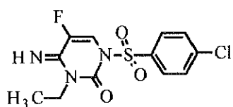
Compound 7:
