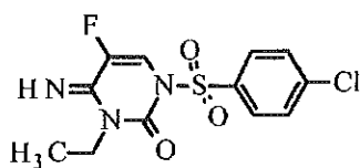
Compound 7:
