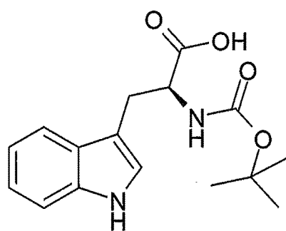
Boc-L-tryptophan
