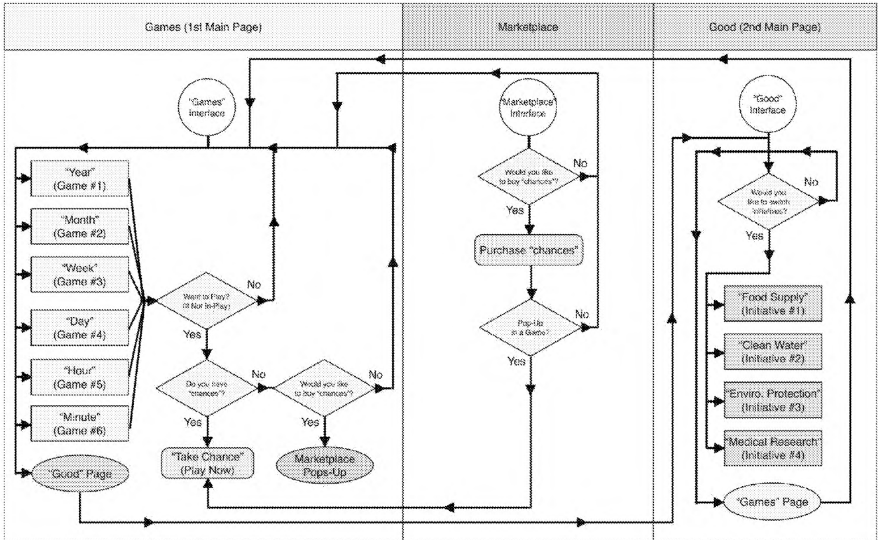
Fig. 3: Mobile App: User Interface FlowChart
