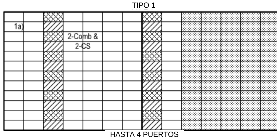
FIG. 2 DL-DMRS-len = 1, DL-DMRS-add-pos = 1, and DL-DMRS-config-type = 1
