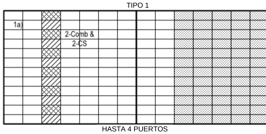
FIG. 1 DL-DMRS-len = 1, DL-DMRS-add-pos = 1, and DL-DMRS-config-type = 1
