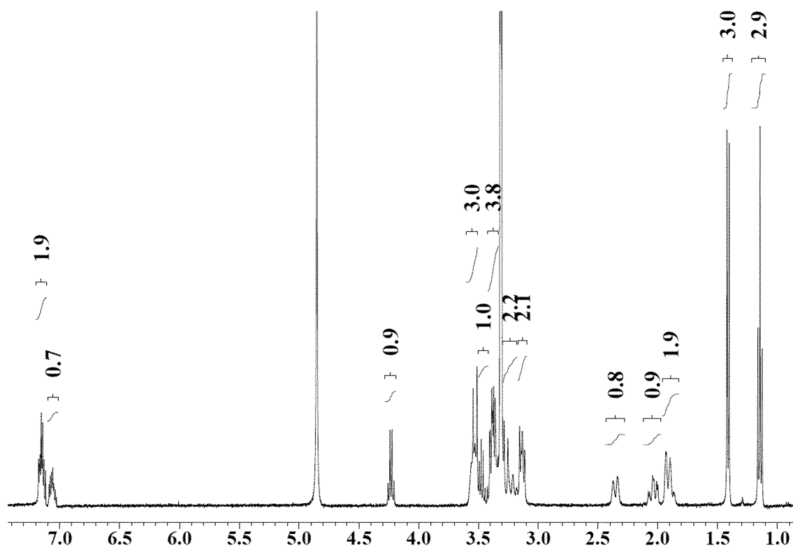
Figure 41: ^1\text{H-NMR} ( d_4\text{-MeOH} , 400 MHz) of oxalate salt Form P2.
