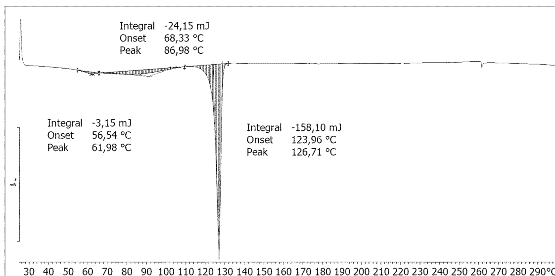
Figure 48: DSC analysis of esylate salt Form P1. Two broad endothermic events at 56 °C and 68 °C are observed prior the melting of the potential esylate salt Form P1 at 124°C (onset). The nature of the two first events is not clear with the available data.
