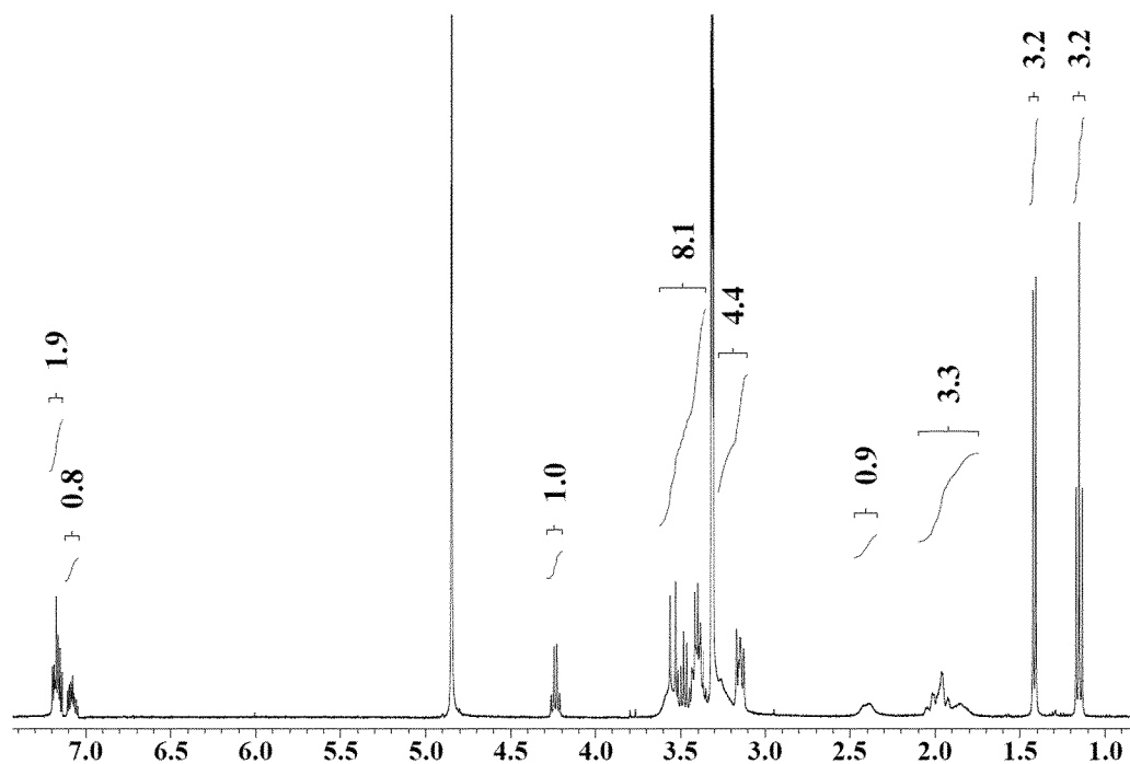
Figure 13: 1 H-NMR ( d 4 -MeOH, 400 MHz) of hydrobromide salt Form P1.
