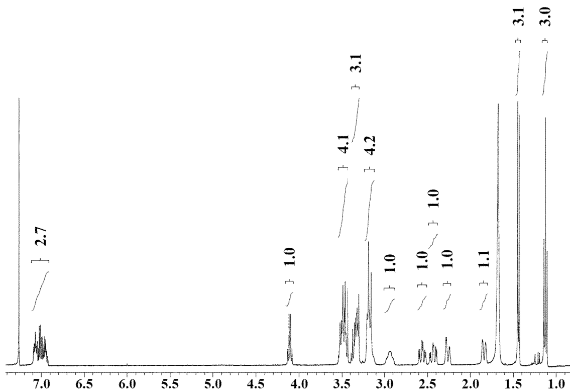
Figure 6. 1 H-NMR ( d -CHCl 3 , 400 MHz) of hydrochloride salt form P2.
