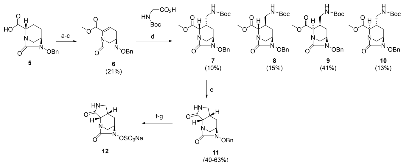
Scheme 1. Synthesis of Compound 12 by Photoredox Coupling a
