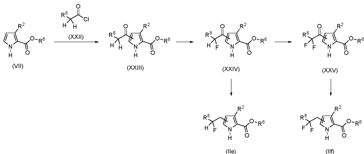
Scheme 7
