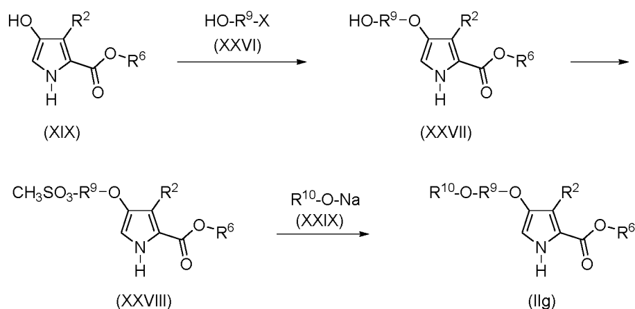
Scheme 8
