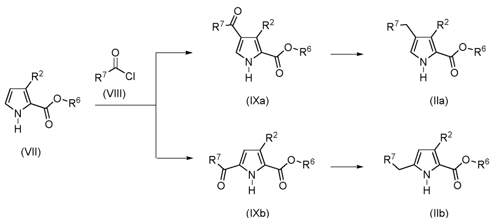
Scheme 2
