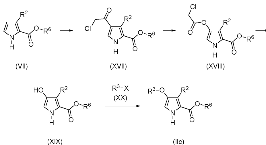
Scheme 5
