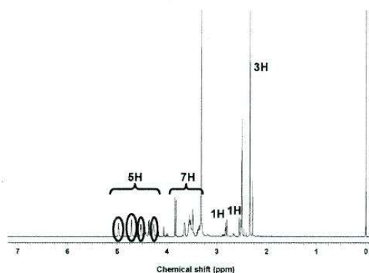
Fig. 3. ^1\text{H} -NMR Spectrum of the Reaction Product between Formaldehyde and Meglumine
