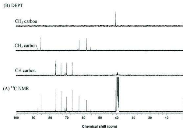
Fig. 4. (A) ^{13}\text{C} -NMR and (B) DEPT Spectra of the Reaction Product between Formaldehyde and Meglumine
