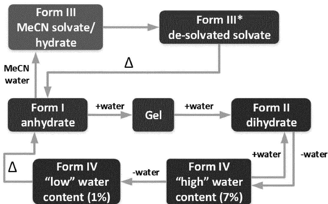
Scheme 3
