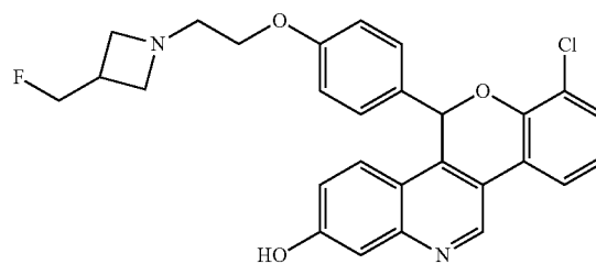
7-chloro-5-(4-{2-[3-(fluoromethyl)azetidin-1-yl]ethoxy}phenyl)-5H-[1]benzopyrano[4,3-c]quinolin-2-ol
