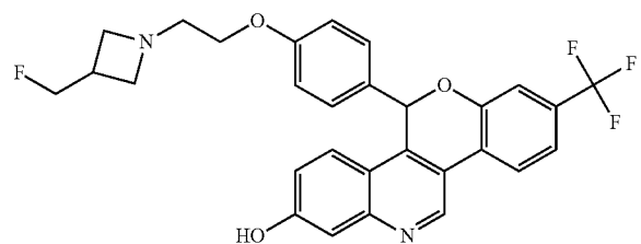
5-(4-{2-[3-(fluoromethyl)azetidin-1-yl]ethoxy}phenyl)-8-(trifluoromethyl)-5H-[1]benzopyrano[4,3-c]quinolin-2-ol
