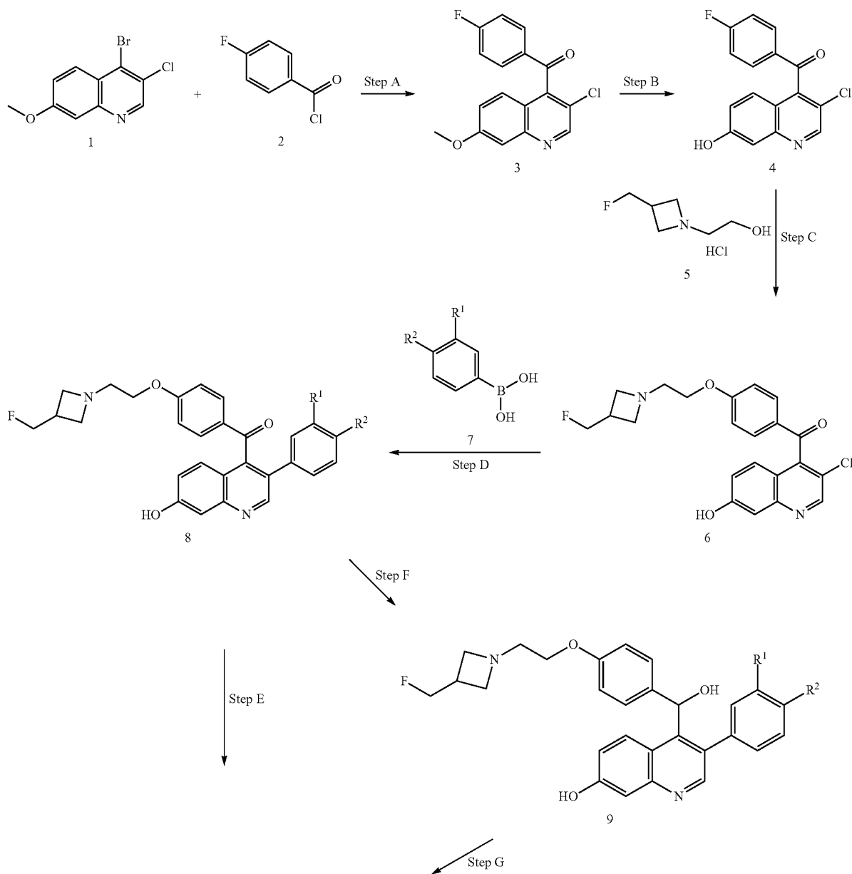
Scheme 1
