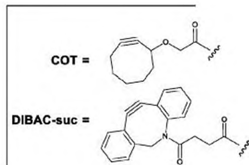
L-1a,b,d,e a , m = 1 , T = \text{COT} b , m = 1 , T = \text{DIBAC-suc} d , m = 0 , T = \text{COT} e , m = 0 , T = \text{DIBAC-suc} L7-P11-1, L17-P11-1, L6-P11-9, y L6-P11-13 (véase Tabla 3)
