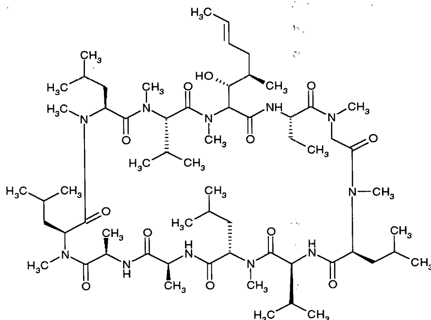
Formula I
