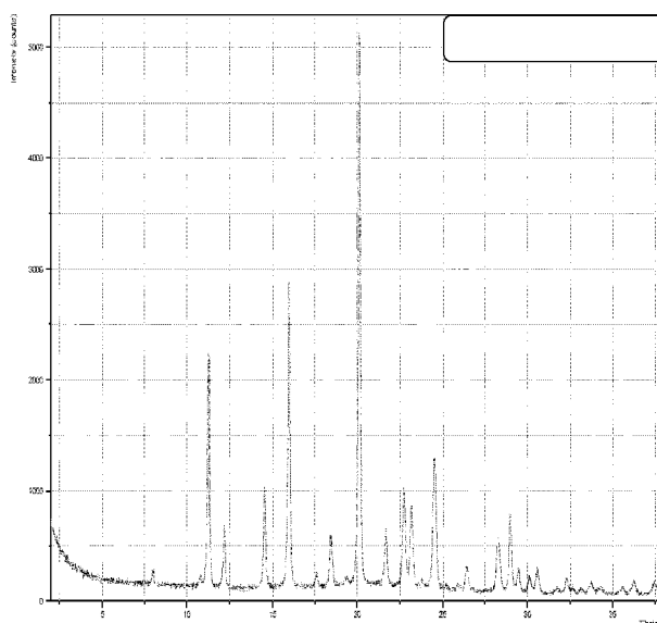
Fig. 1: X-ray diffraction pattern of I-2 (Mod. A)
