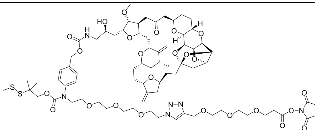
NHS-PEG3-triazol-PEG3-disulfuro-PAB-eribulina (ER-001244129)
