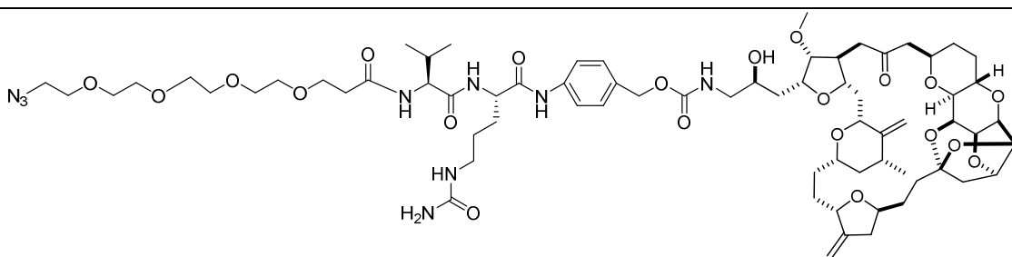
PEG4-Val-Cit-PAB-eribulina
