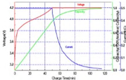
Charge Specialty
