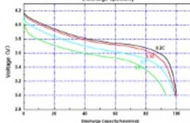
Discharge Specialty
