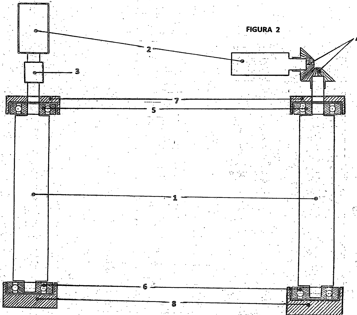
VISTA FRONTAL
