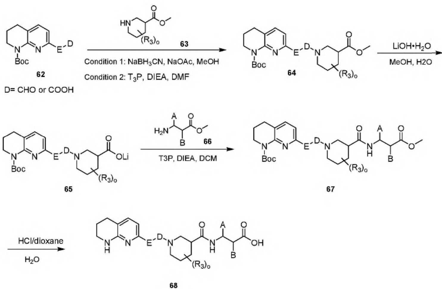
Scheme 14
