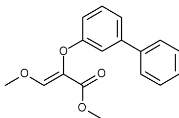
methyl (Z)-3-methoxy-2-(3-phenylphenoxy)prop-2-enoate
