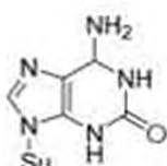
IsoGuanosina IsoG
