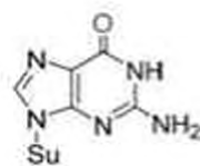
Guanosina G
