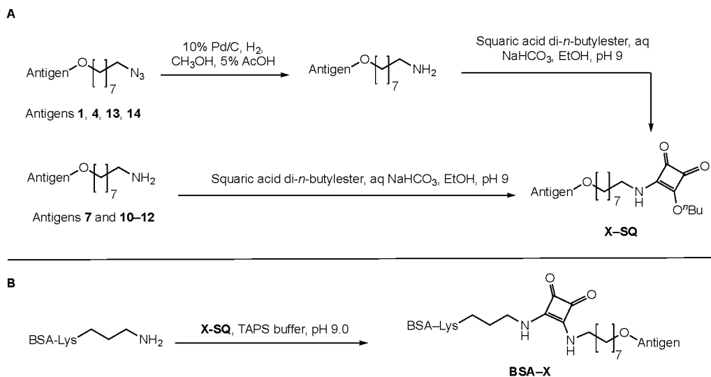
Scheme 13. Conjugation of antigens to BSA. Abbreviations: AcOH = acetic acid; ^n\text{Bu} = n -butyl; EtOH = ethanol; TAPS = ([tris(hydroxymethyl)methylamino]propanesulfonic acid).
