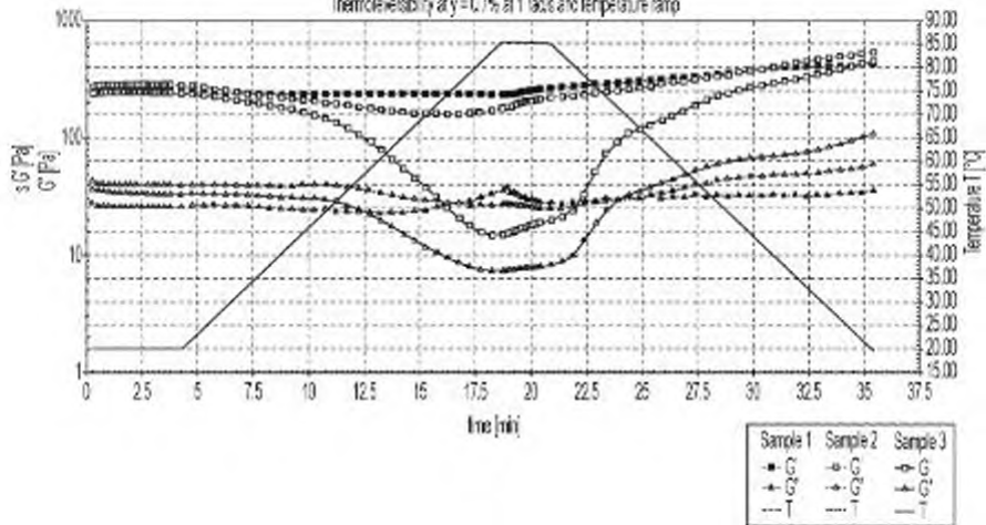
Thermoreversibility at \gamma = 0.7\% at 1 rad/s and temperature ramp
