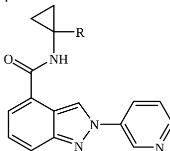
Formula II
