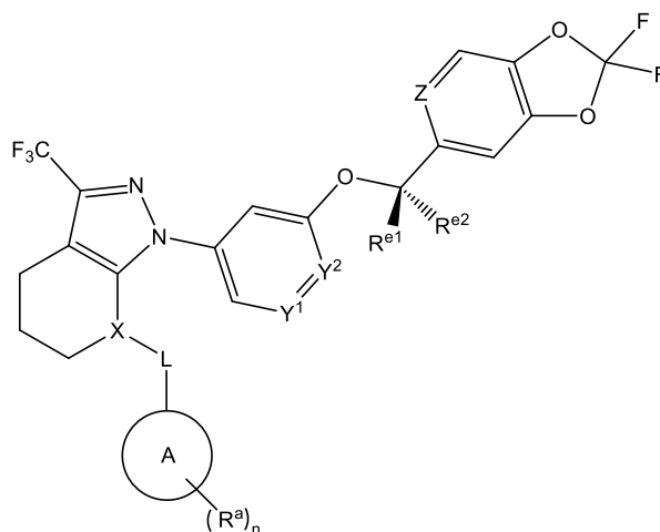
(I-a'),
