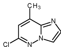
(Compound X-1)
